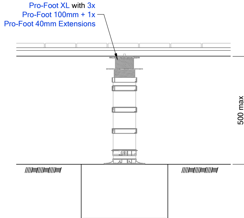
Typical Pro-Foot pedestal System - 500mm Maximum Height Assembly
